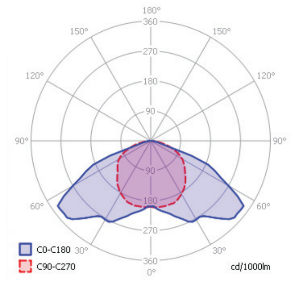
BEAM ANGLE 140°
